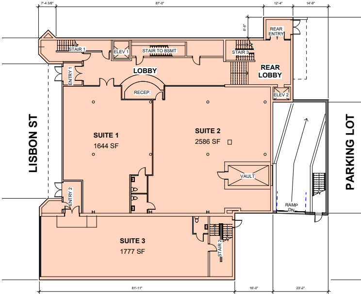
1 | FIRST FLOOR PLAN 3/32" = 1'-0"
