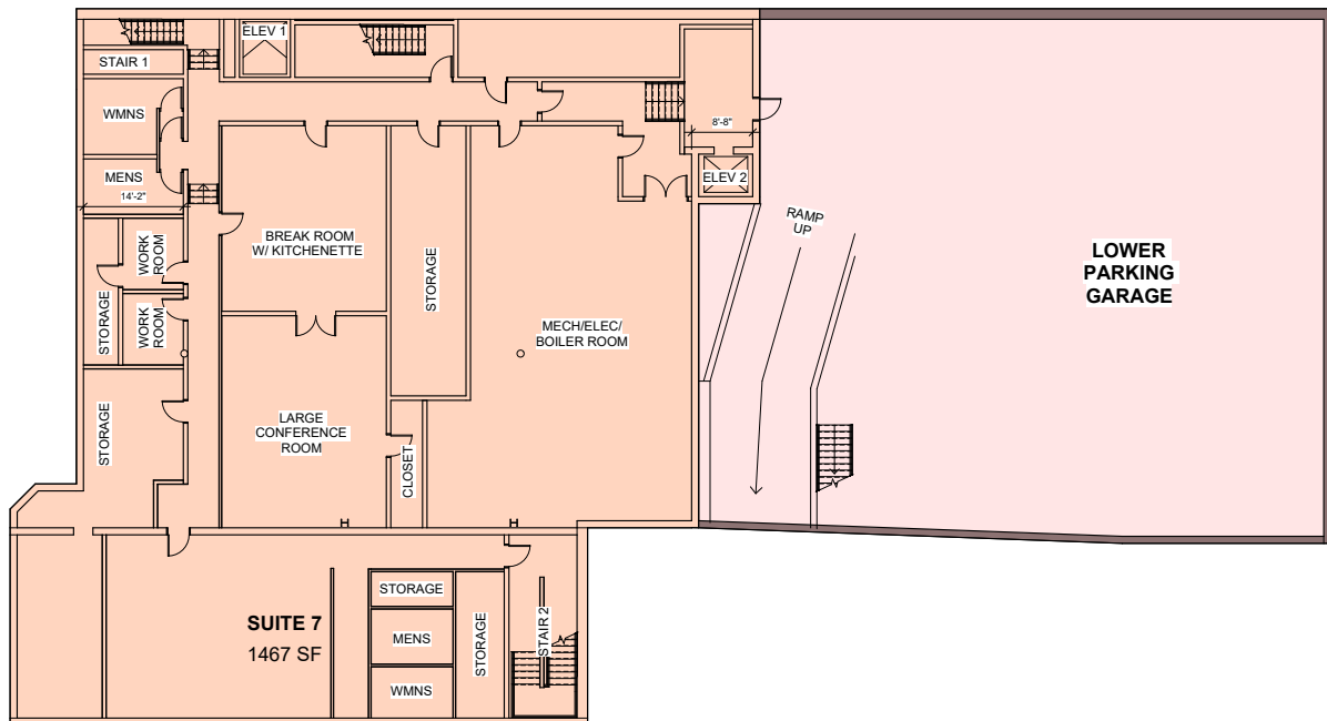
3 | BASEMENT/GARAGE PLAN
